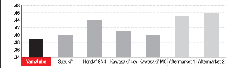
Four Ball Friction Test – 30 minutes
