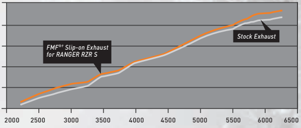
RANGER RZR HORSEPOWER COMPARISON
