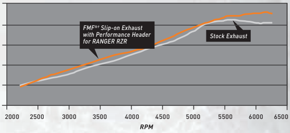
RANGER RZR HORSEPOWER COMPARISON
