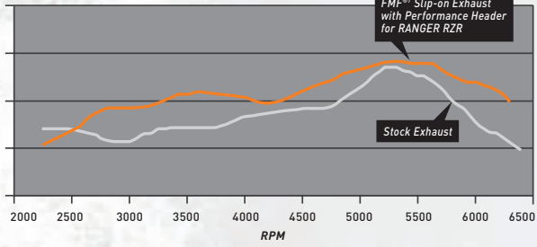
RANGER RZR TORQUE COMPARISON
